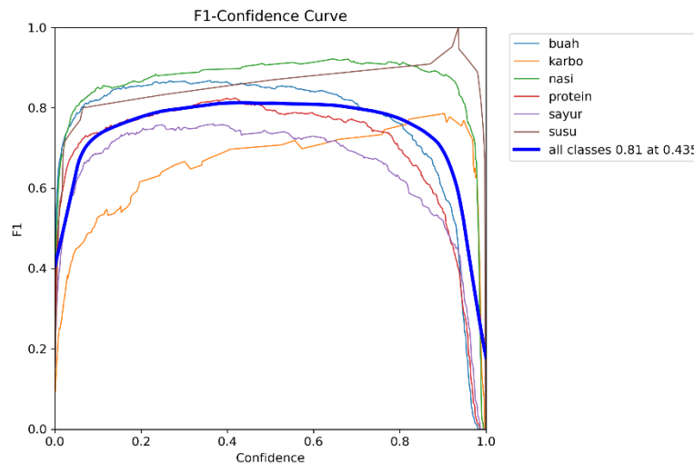
Gambar 5.7. F1-Confidence Curve
