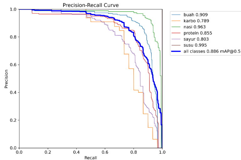
Gambar 5.6. Precision-Recall Curve
