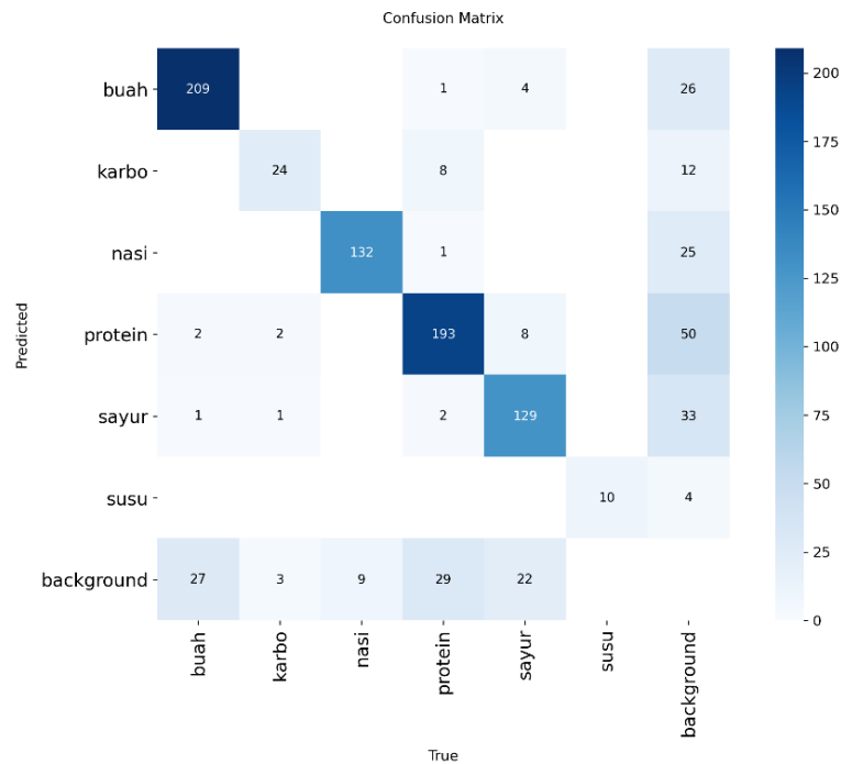
Gambar 5.4. Confusion matrix
